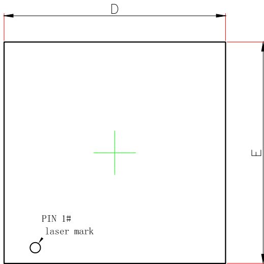
DFN3×3-8L-D (P0.65T0.75)
