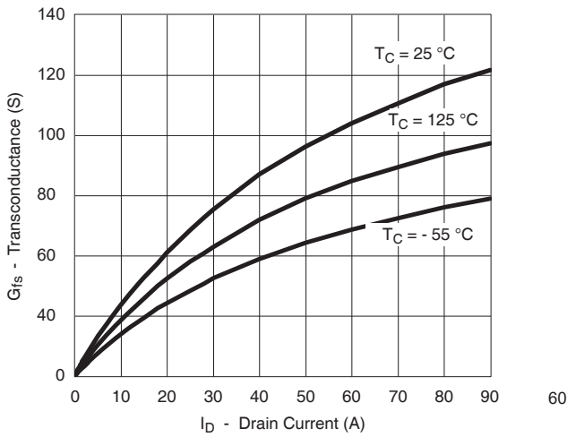
Transconductance
