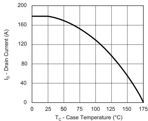
Current De-Rating
