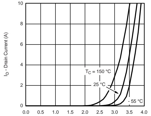
I_D - Drain Current (A) V_{GS} - Gate-to-Source Voltage (V) T_C = 150\text{ }^\circ\text{C} 25 °C -55 °C Transfer Characteristics
