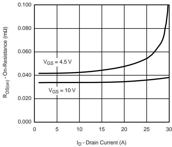
R_{DS(on)} - On-Resistance (mΩ) I_D - Drain Current (A) V_{GS} = 4.5\text{ V} V_{GS} = 10\text{ V} On-Resistance vs. Drain Current and Gate Voltage
