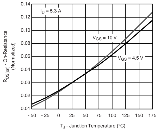
R_{DS(on)} - On-Resistance (Normalized) T_J - Junction Temperature (°C) I_D = 5.3\text{ A} V_{GS} = 10\text{ V} V_{GS} = 4.5\text{ V} On-Resistance vs. Junction Temperature
