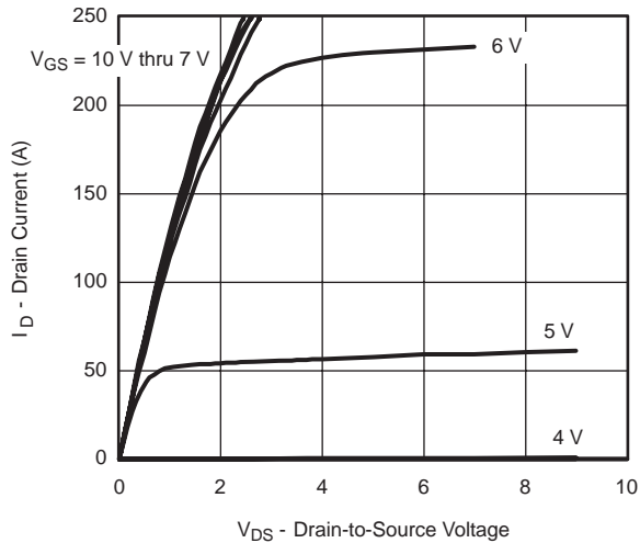
V_{GS} = 10 V thru 7 V Output Characteristics
