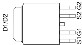
TO-252-4L
