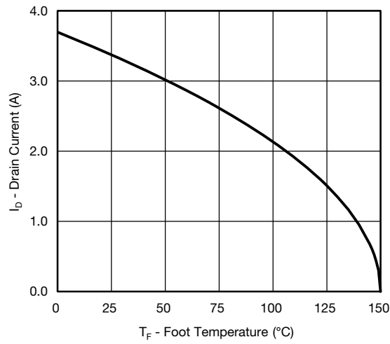
Current Derating*
