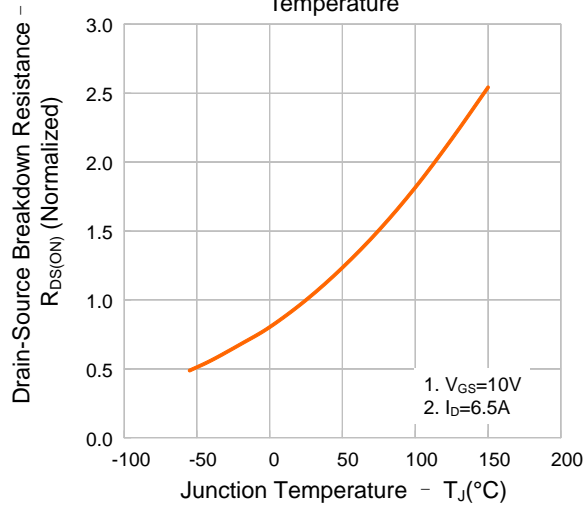
Figure 11. On-Resistance vs. Temperature
