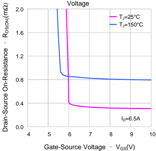
Figure 5. On-Resistance vs. Gate-Source Voltage
