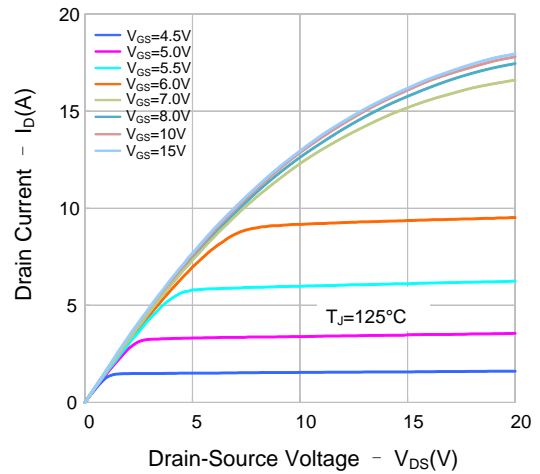
Figure 2. Output Characteristics
