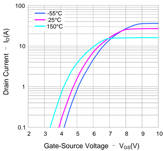
Figure 3. Transfer Characteristics
