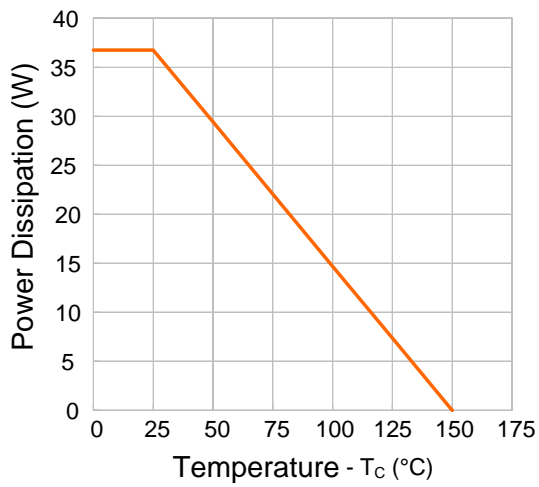
Figure 13. Power Dissipation vs. Temperature
