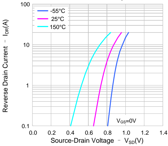
Figure 7. Body Diode Forward Voltage vs. Source Current and Temperature
