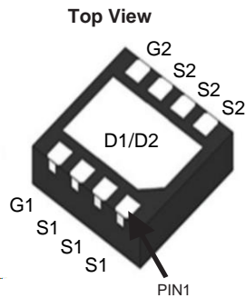
DFN3X3-8L Pin Configuration
