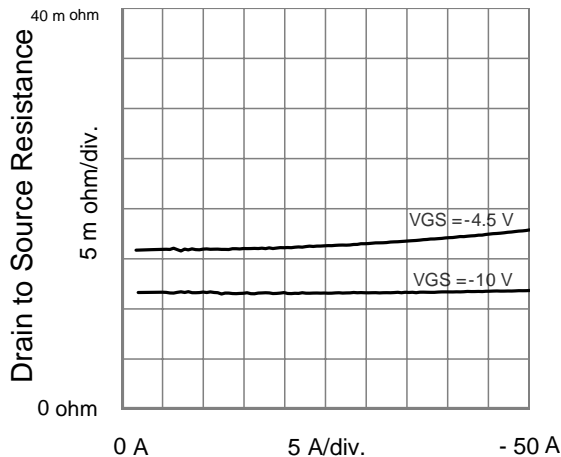
Drain Current
