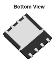
DFN5X6-8L Pin Configuration
