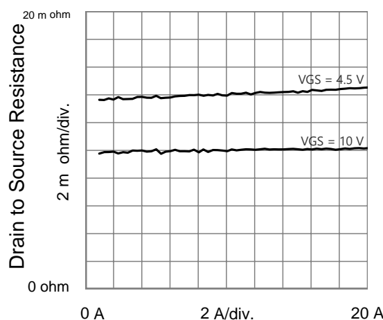
Drain Current
