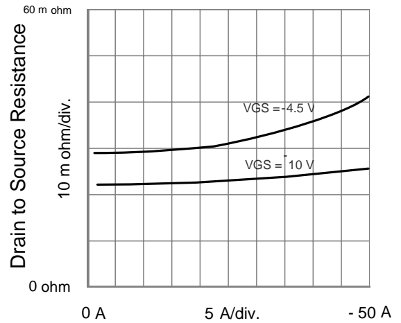
Drain Current
